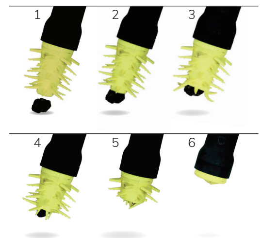
Corium sample recovery simulation
